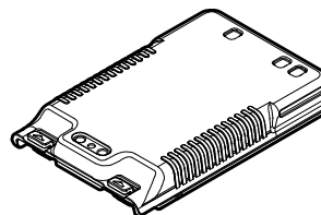
Long life lithium-ion battery pack (SBR-14LI: 7.2V, 2,200 mAh)
