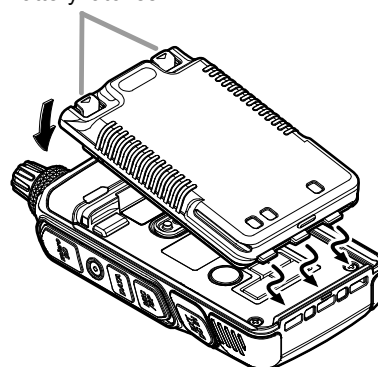
Battery latches
